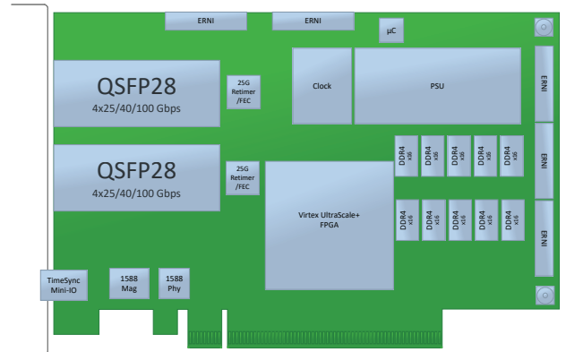
2-port 200G PCIe SmartNIC NT200A02
