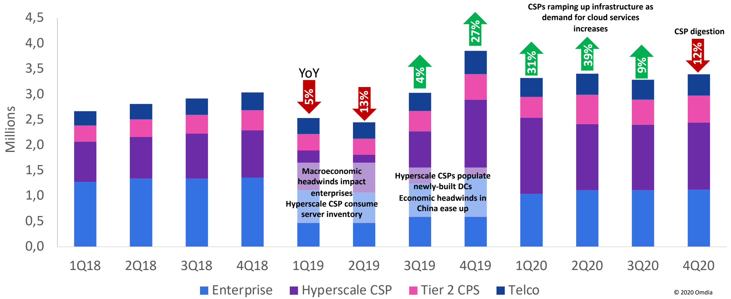
Quarterly server shipments
